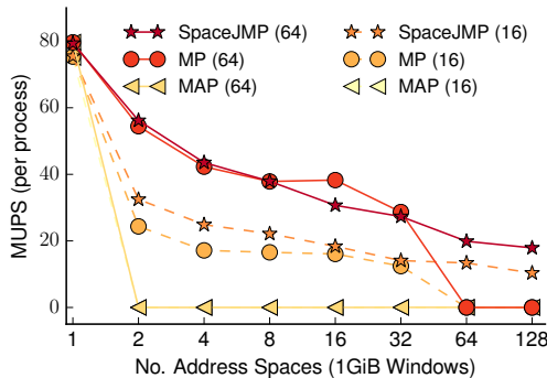
Figure 8: Comparison of three designs to program large memories with GUPS ( M3 ). Update set sizes 16 and 64.
